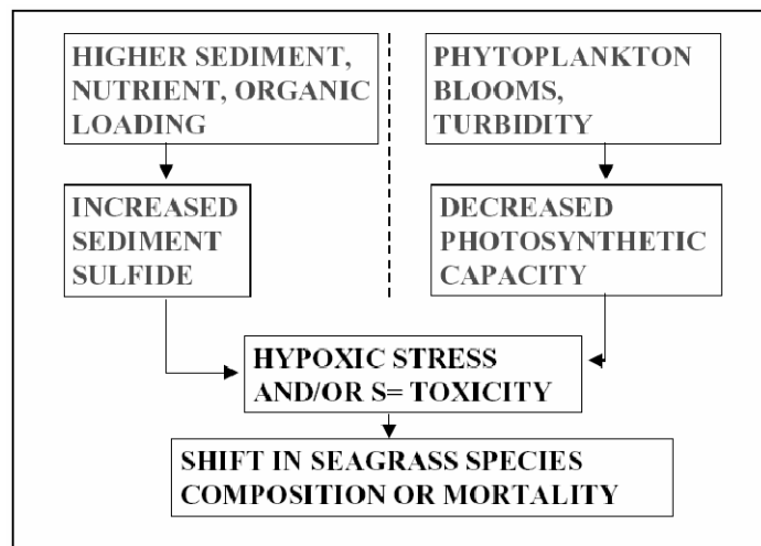
Figure 4. Factors affecting the vulnerability of eelgrass to sulfide toxicity.
