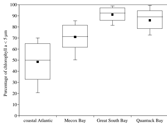
Figure 3. A comparison of the percentage of chlorophyll passing through a 5 µm mesh from samples collected in the coastal Atlantic Ocean (2002), Mecox Bay (2002), Great South Bay (1998 – 2002), and Quantuck Bay (1999 – 2002). Note: Mecox Bay is a temporally open estuary on the south shore of Long Island which exchanges with the Atlantic Ocean and is located 5 km east of Shinnecock Bay within LISSE.
